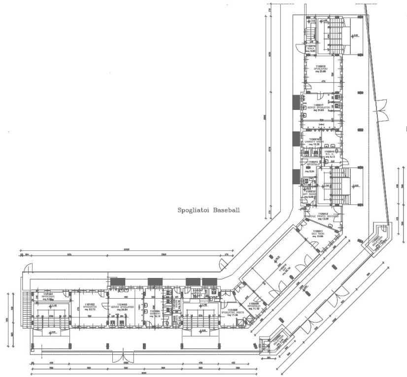
Piano Terreno
