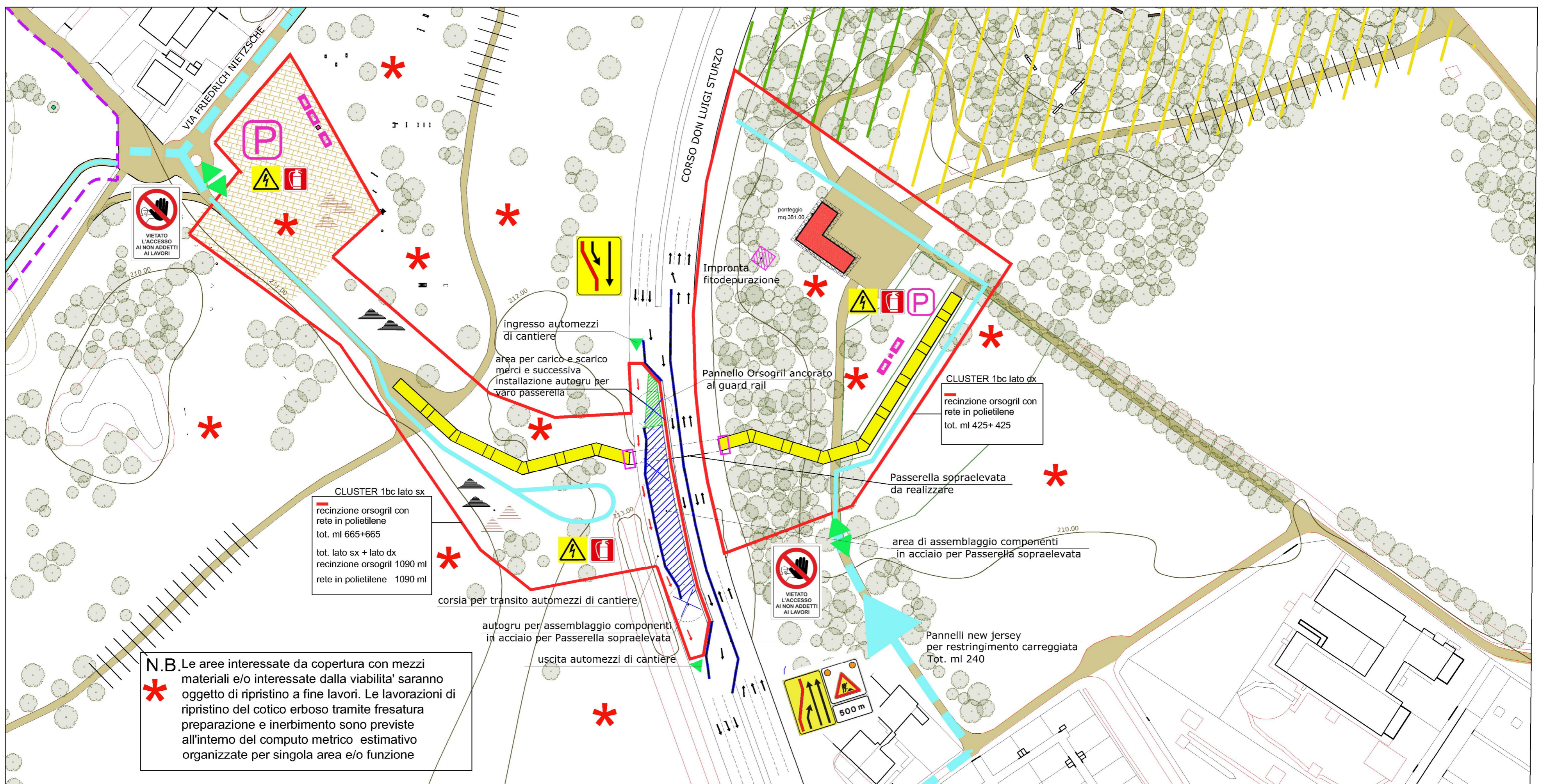
PLANIMETRIA AREA - KEYPLAN AREE CANTIERE _ Scala 1:5000
