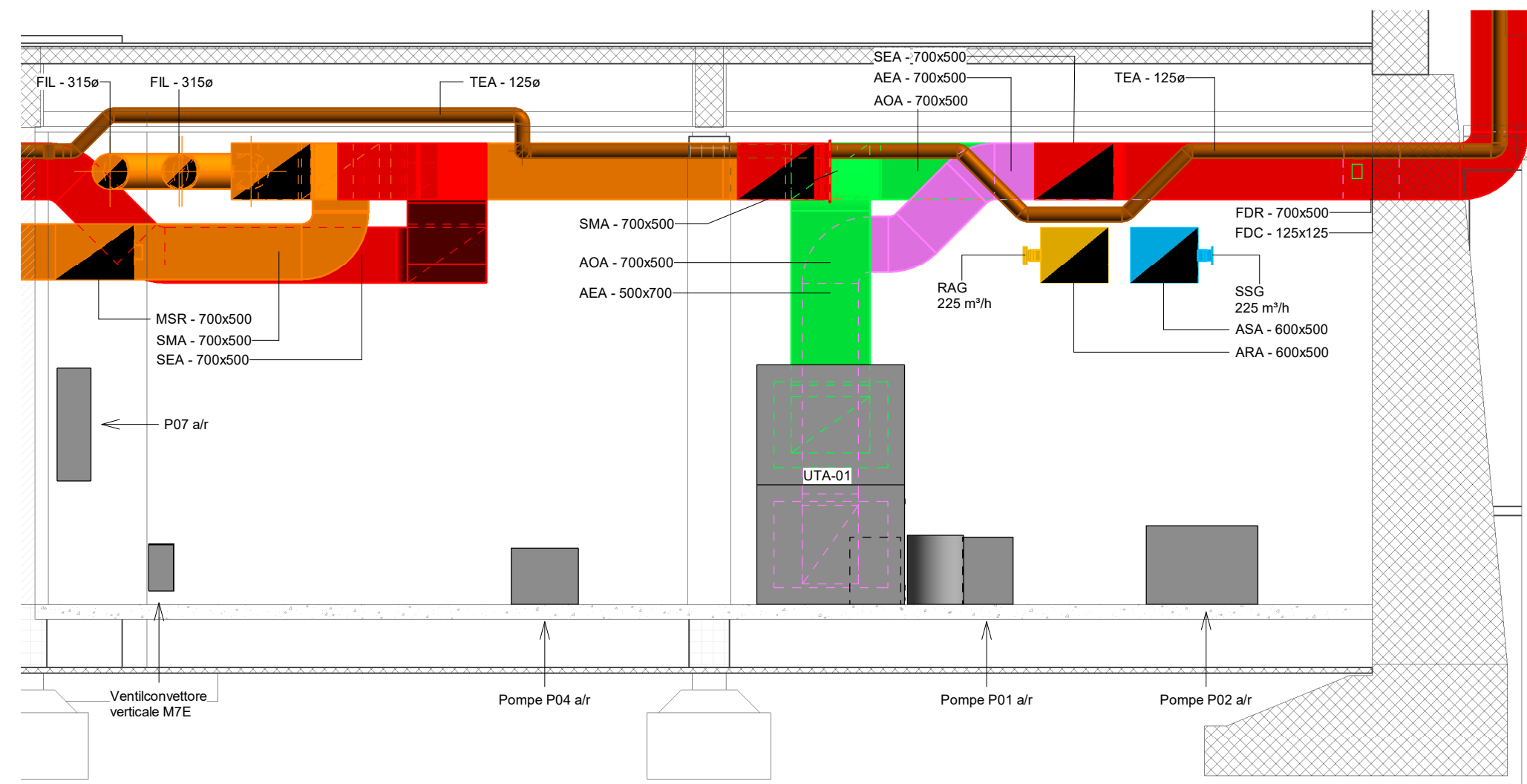
5 CLI Section_2 1:50
