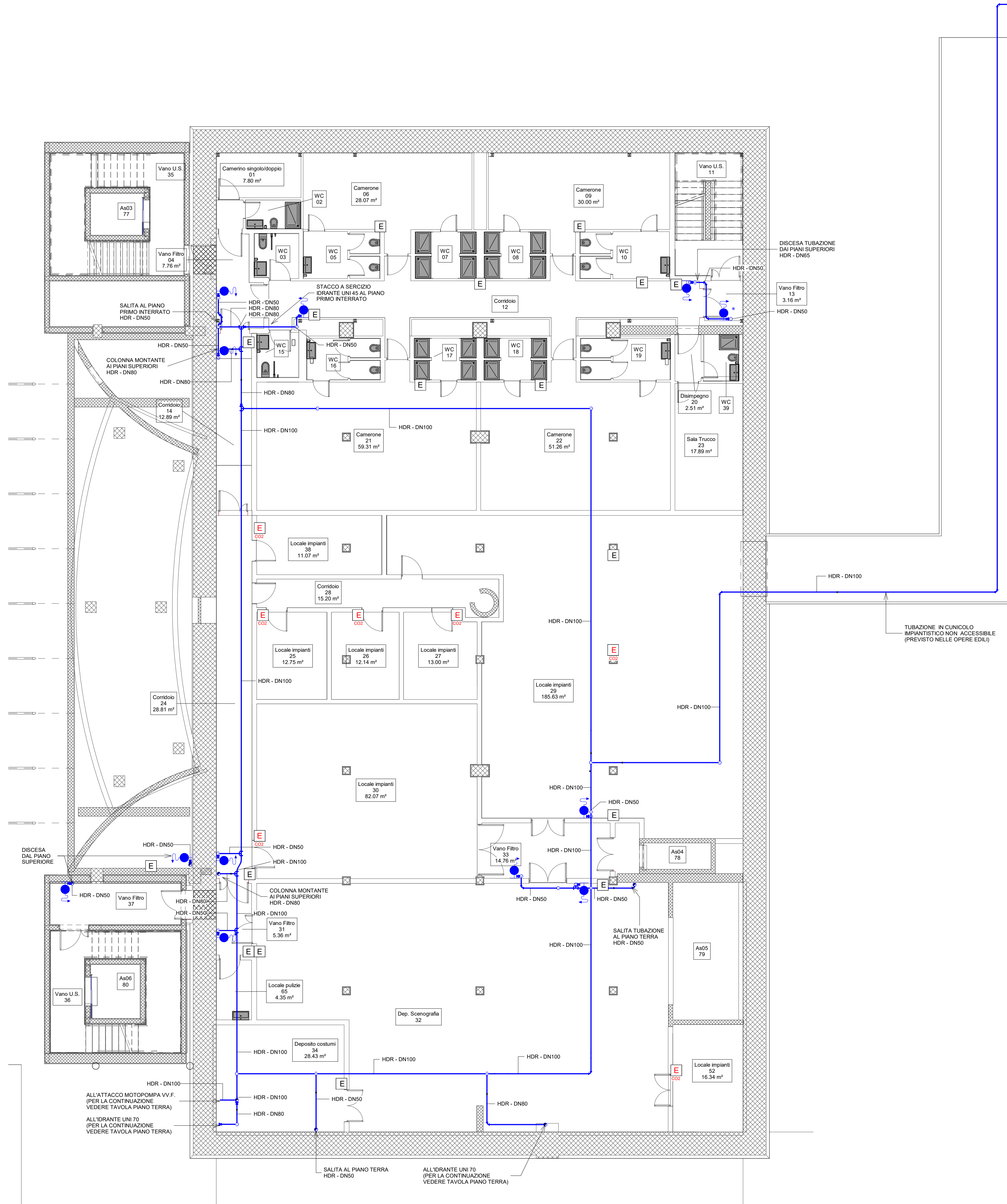
1 Pianta piano interrato -2 1 : 100
