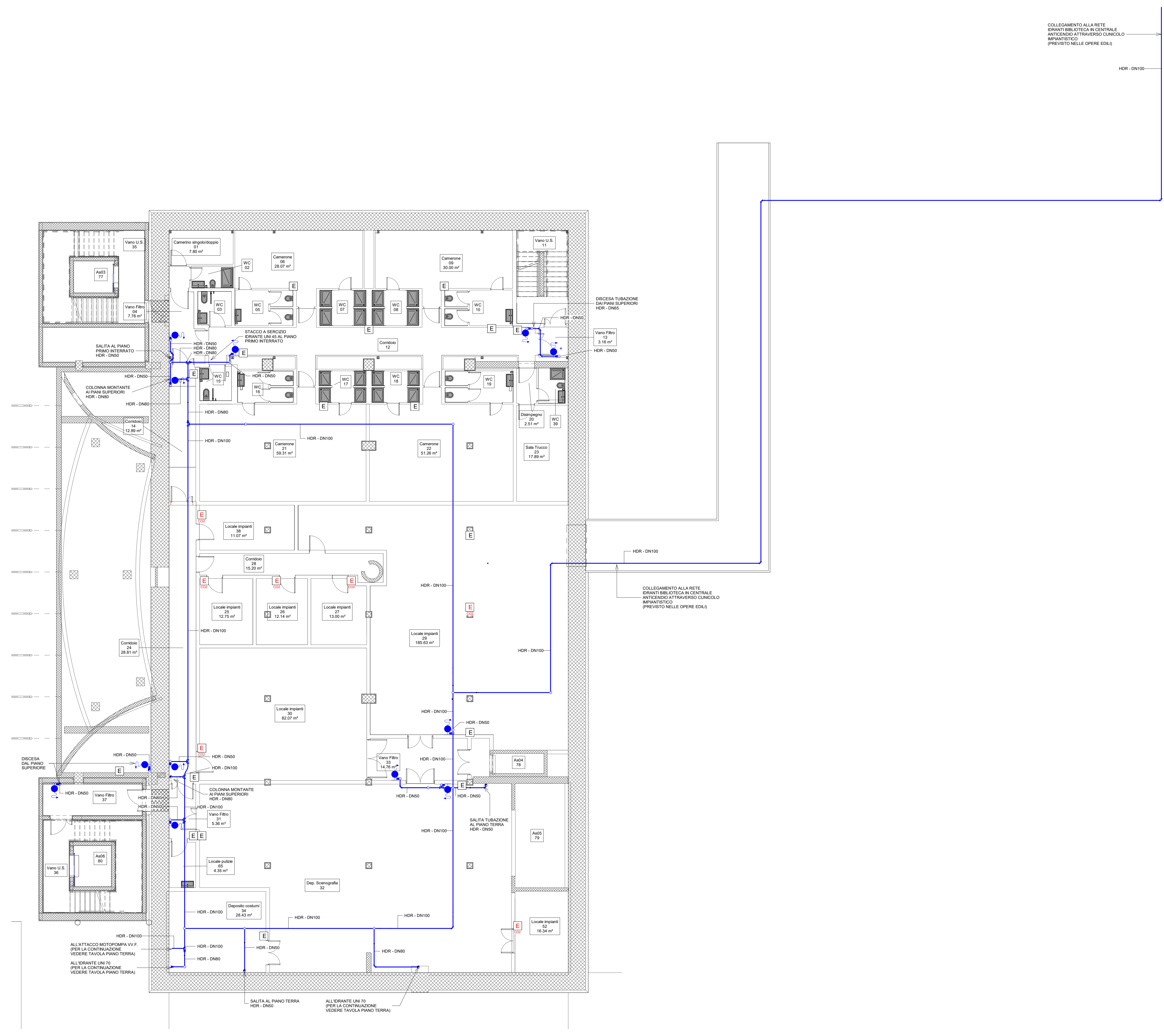
1 Pianta piano interrato -2 1 : 100
