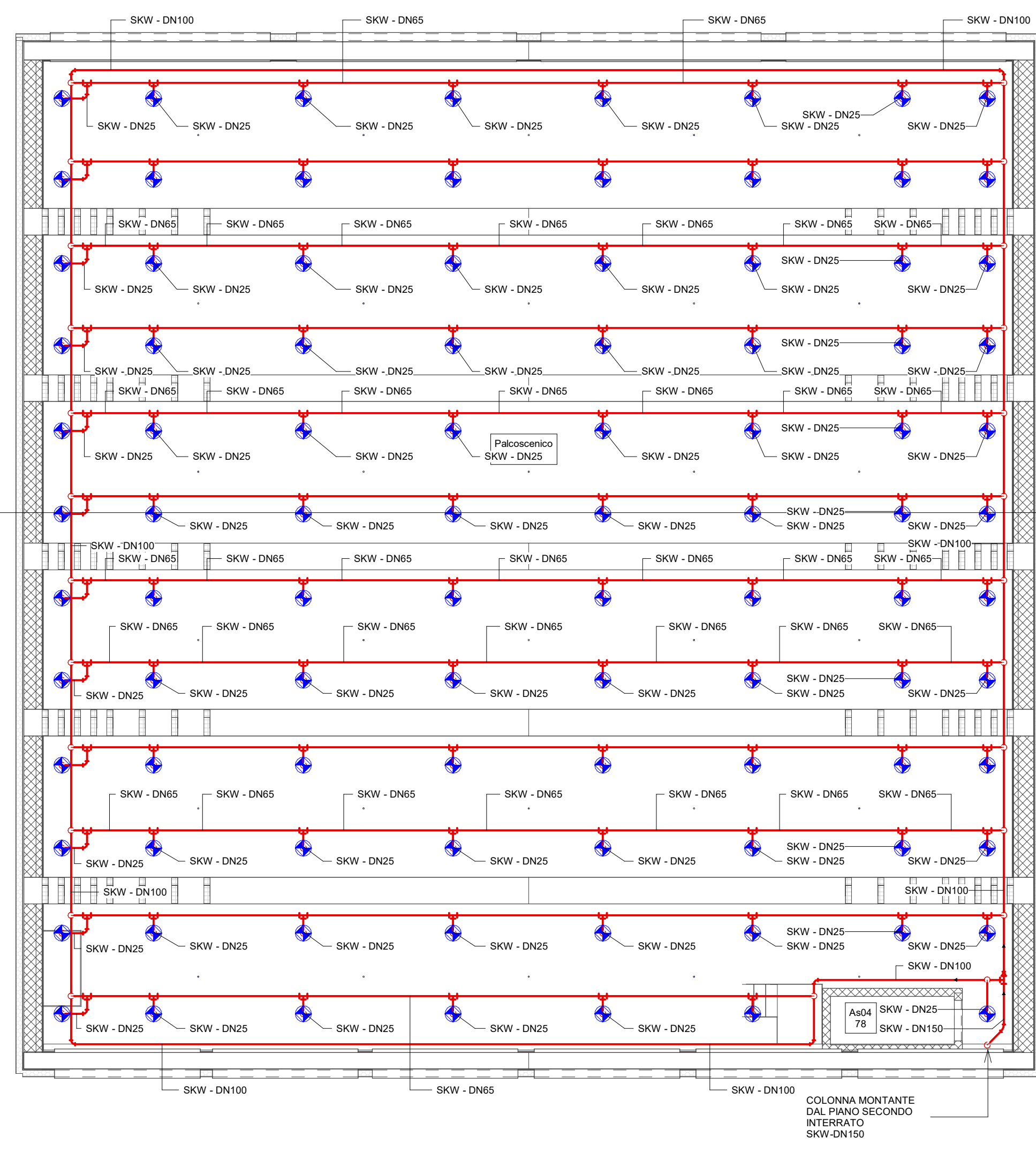
4 Piano Torre scenica sopra graticcio 1 : 100
