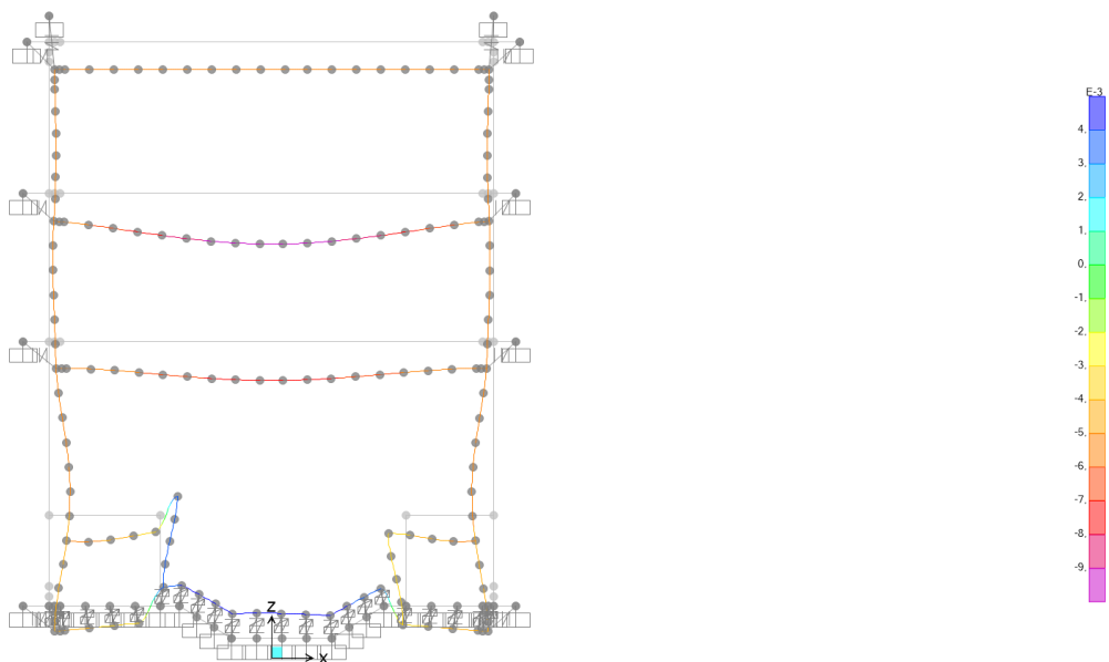
Figura 81.DEFORMATA SLE RARA
