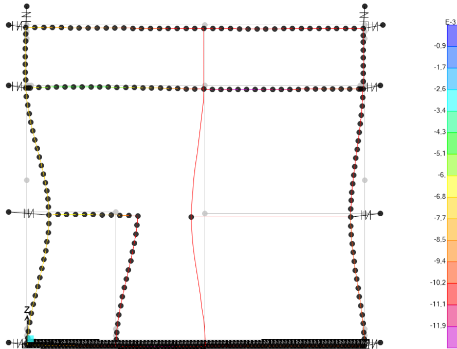
Figura 62.DEFORMATA SLE RARA
