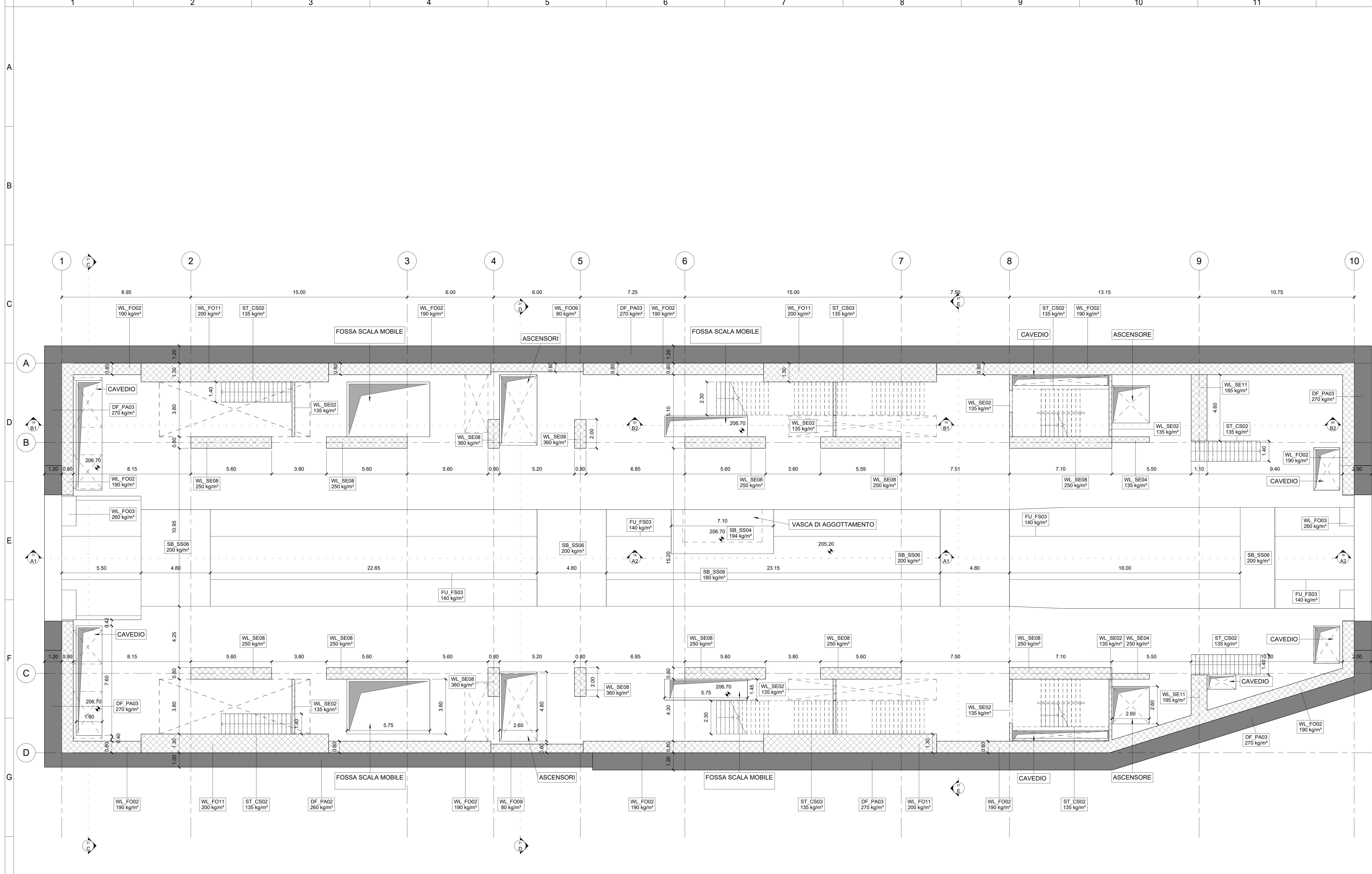
H 1 PIANO BANCHINA 1:100
